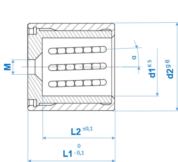
BALL BUSH CENTERER
