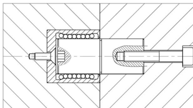
Assembly, option n°2
