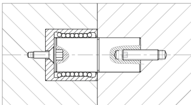
Assembly, option n°1
