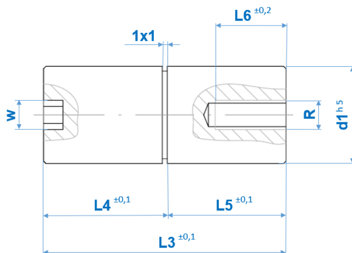
PILLAR BALL CENTERER
